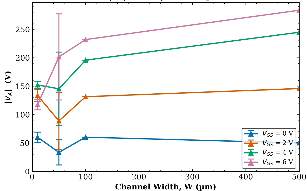
TFT1 Combined (Tr. 1 & 2) |V_A| vs W | L = 80\text{ }\mu\text{m}
